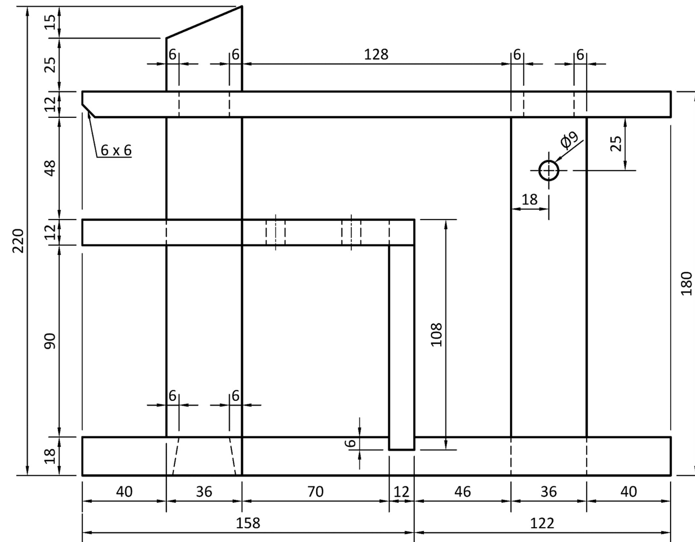
Elevation/Aghaidhchló
